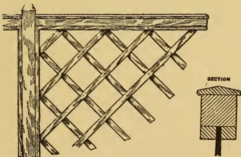
Fig. 61.—Construction of trellis screen
